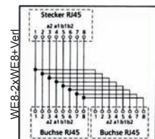
MP8(8)-2xMJ8(4),cable-sharing
